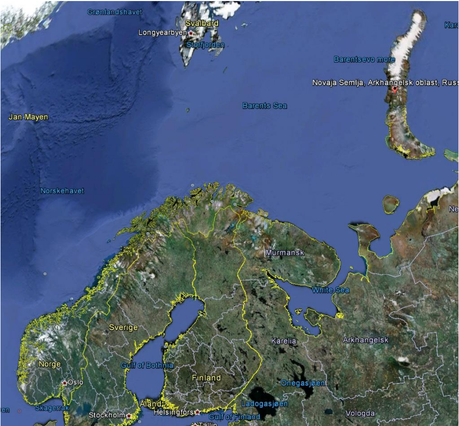
Figure A2: Test Site in Novaya Zemlya (Russia)
