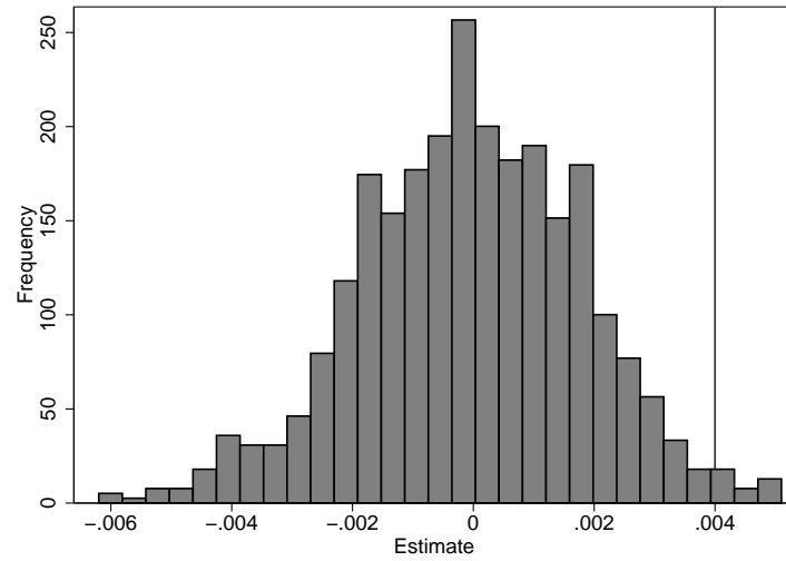
Figure A4: Randomization Inference for Simulated Benefit Estimates (Table A4)
